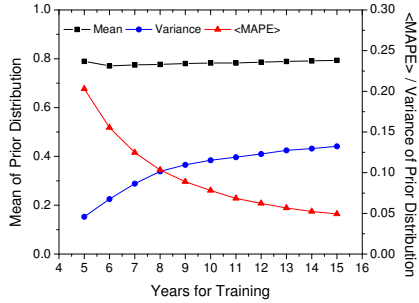
Figure 5: Effect of training period length.
