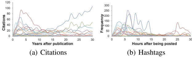
Figure 1: Stochastic Popularity dynamics. (a) 20 papers randomly selected from Physical Review during 1960s. (b) 20 Hashtags randomly selected from Twitter in 2012.
