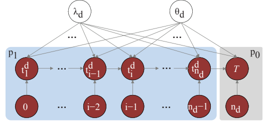
Figure 2: Graphical representation of the generative model for popularity dynamics via reinforced Poisson process.
