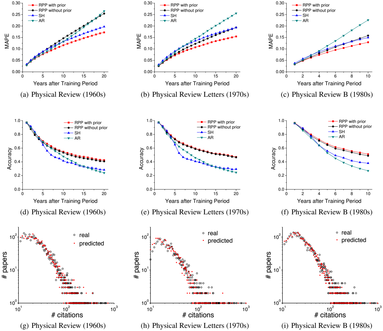
Figure 4: The performance comparison in popularity prediction.
