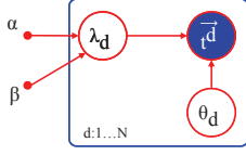
Figure 3: Probabilistic graphical model for reinforced Poisson process with conjugate prior.
